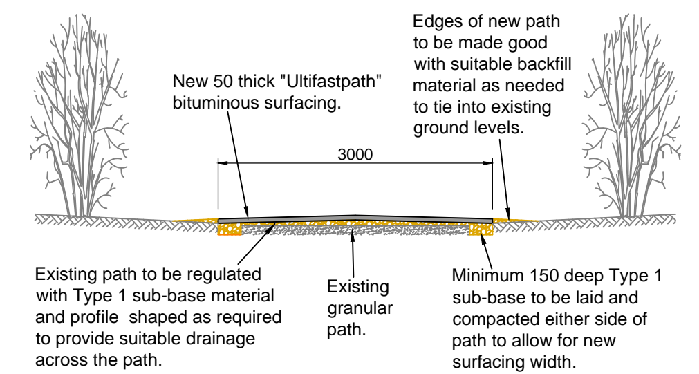
Typical 3m Wide Path Construction (2m & 2.5m Wide Path Constructions Similar)
