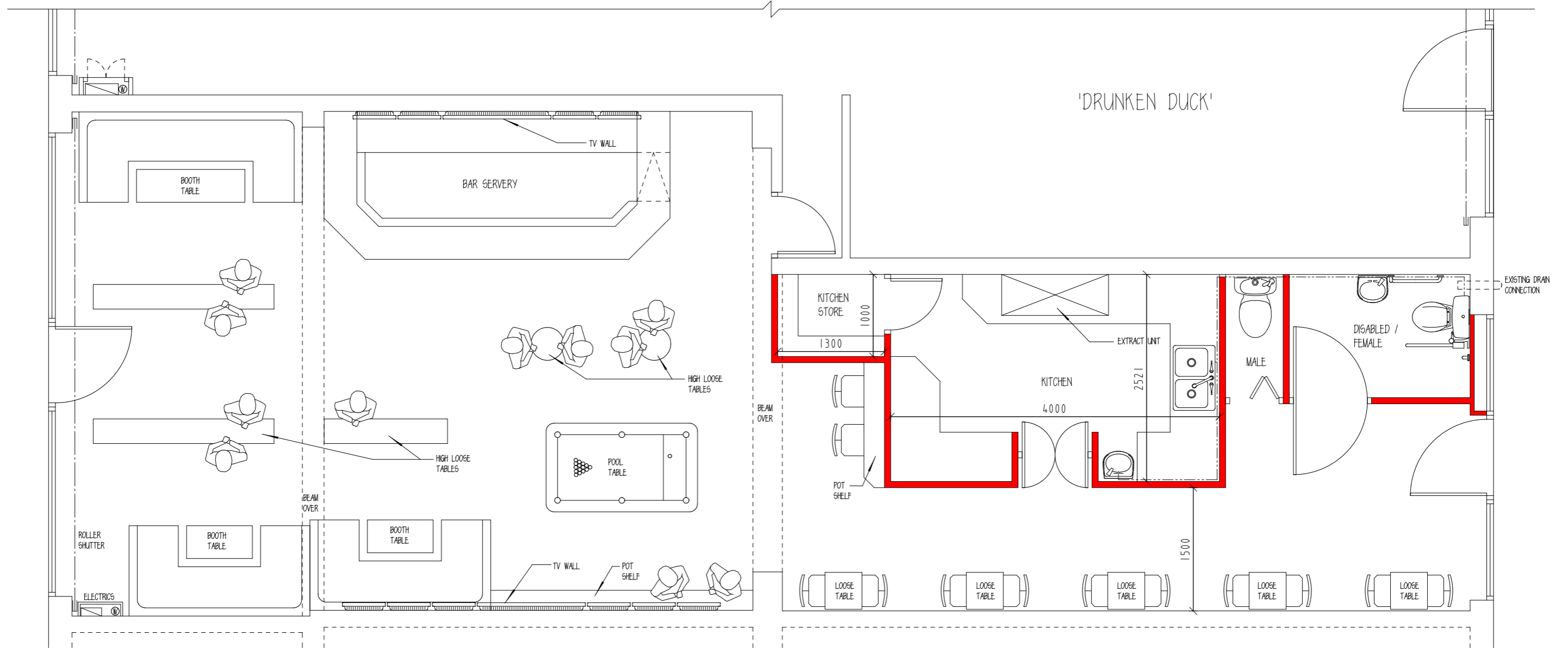
JULY 2022 - PROPOSED FLOOR PLAN - 1:50 AT A3
